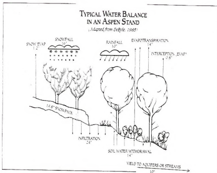
Figure 1. Water balance in a typical western aspen stand (DeByle 1985a).
